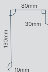
FOLDED BARGE/GABLE
