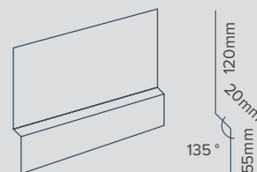
FOLDED Z - FLASHING
