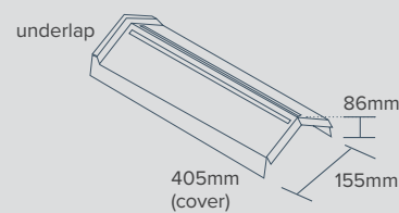
RIDGE CAP
