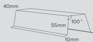
FOLDED RIDGE/HIP
