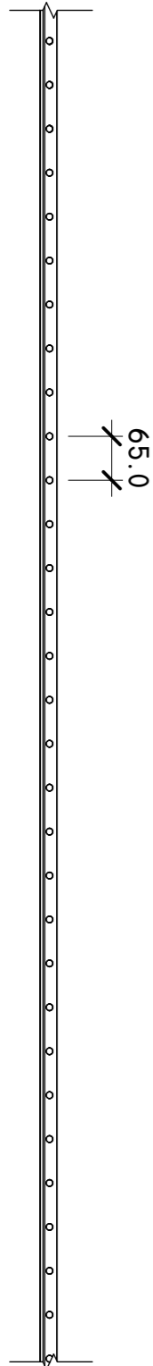
SIDE HOLE SPACING 1:10@A3 FOR SIGMA BATTEN
