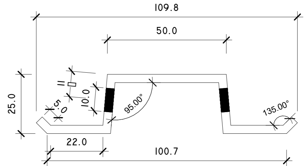
CROSS SECTION 1:1@A3
