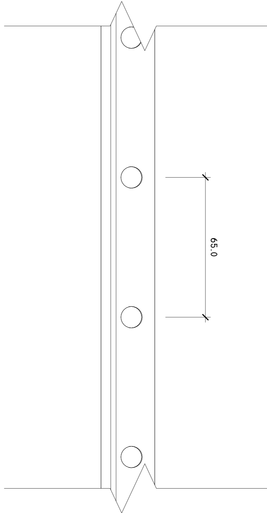
SIDE HOLE DIMENSIONS 1:1@A3 FOR SIGMA BATTEN
