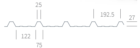
Figure 1: Profile Dimensions (nominal)
